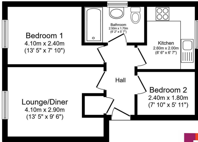
Floor Plan Floor area 38.6 sq.m. (416 sq.ft.)
